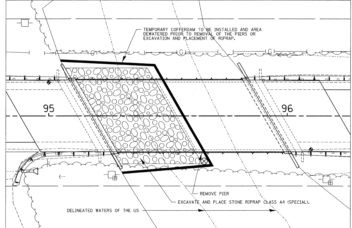
STONE RIPRAP CLASS A4 PLACEMENT - PHASE I
