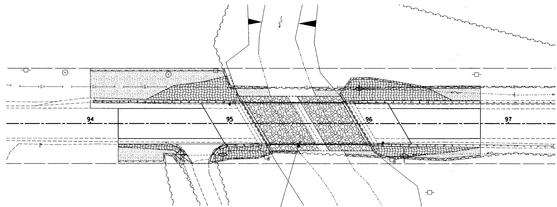
STONE RIPRAP CLASS A4 PLACEMENT - PHASE I
