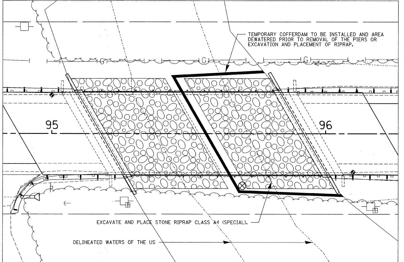
STONE RIPRAP CLASS A4 PLACEMENT - PHASE II
