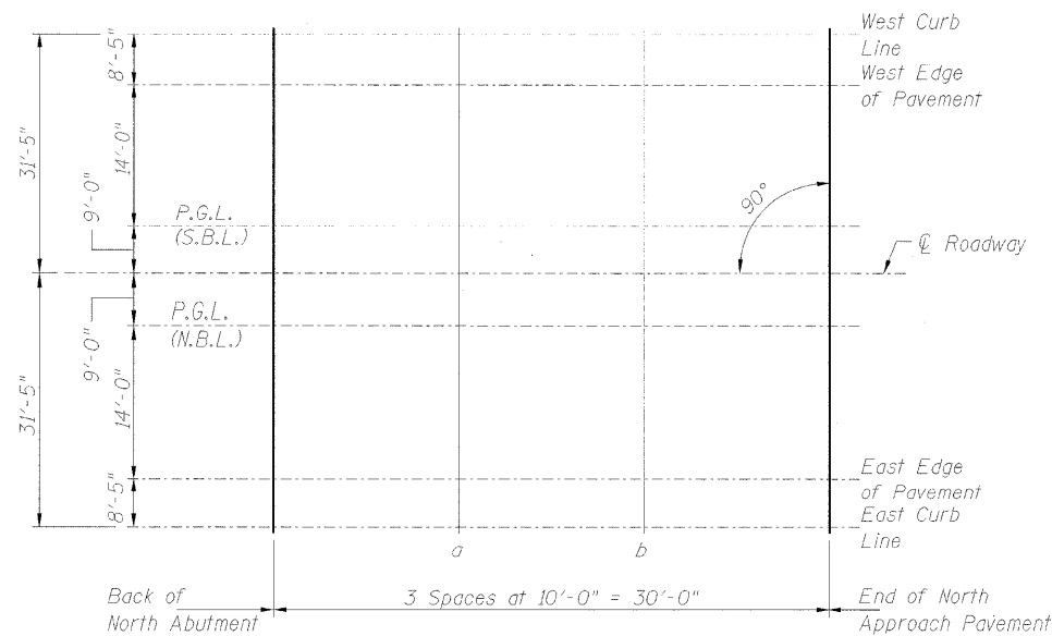
DIAGRAMMATIC PLAN
