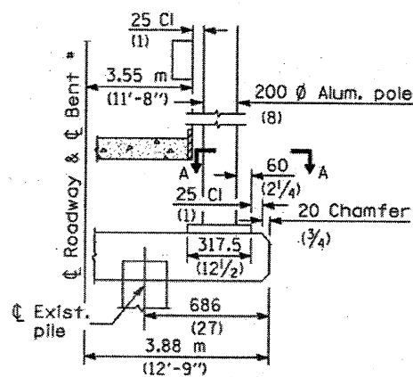
BENT # (Looking )
