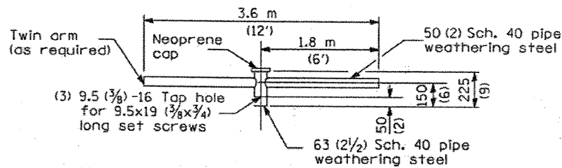
TENON MOUNT BRACKET ARM
