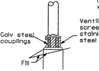
BREAKAWAY COUPLING
