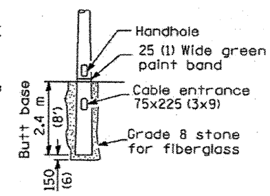
BUTT BASE
