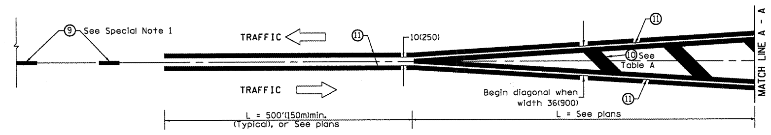
MEDIAN INTRODUCTION - WIDTH TRANSITIONS
