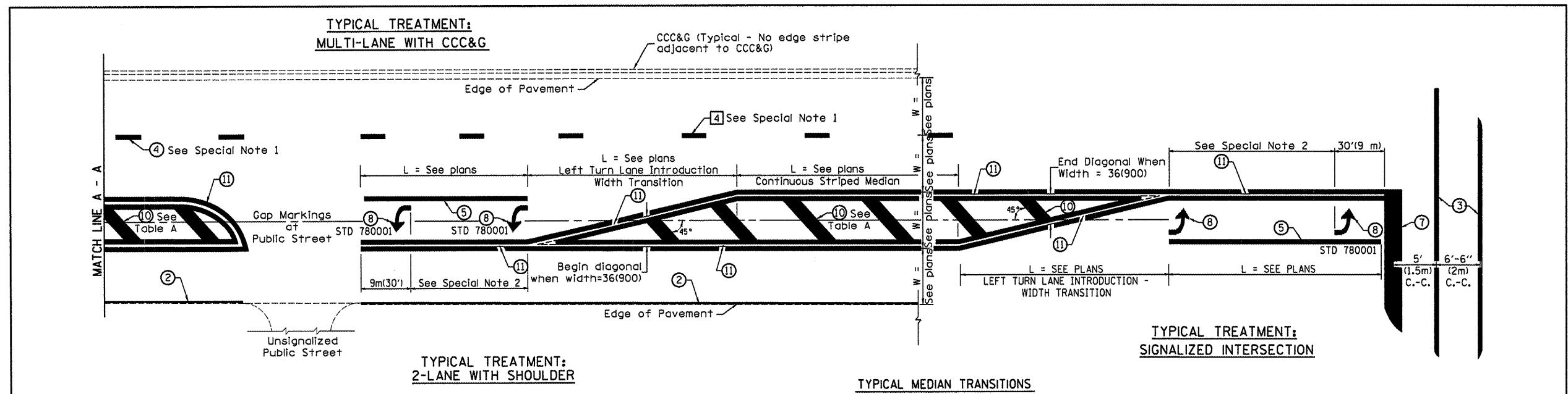
TYPICAL MEDIAN TRANSITIONS
