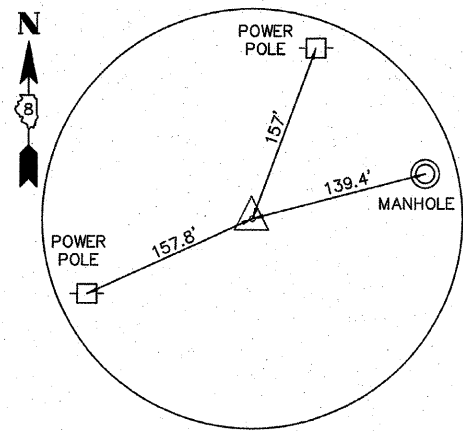
BOWLER ROAD POT STA 10+00.00
