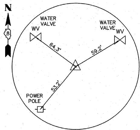
NORTH SEVEN HILLS ROAD/WEIL ROAD POT STA 379+03.52
