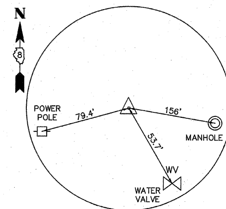
BOWLER ROAD PT STA 12+79.64
