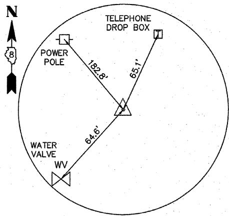
BETHEL SCHOOL ROAD PT STA 40+73.65
