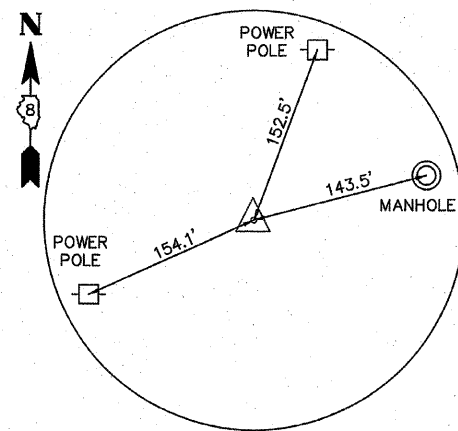
BOWLER ROAD PC STA 10+07.40
