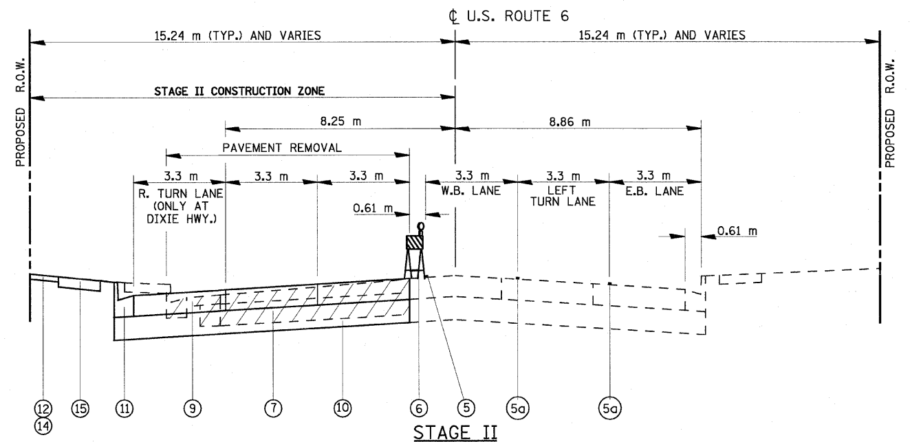
STAGE II U.S. ROUTE 6 (159th STREET) DIXIE HIGHWAY TO WOOD STREET
