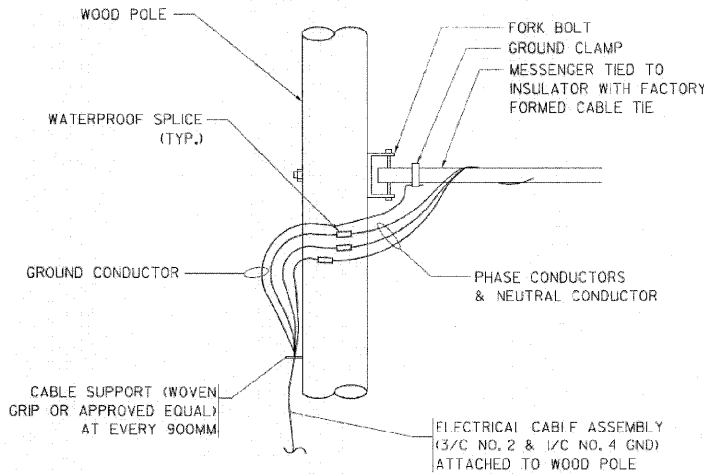
AERIAL CABLE CONNECTION DETAIL
