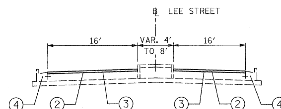
PROPOSED TYPICAL SECTION STA. 300+32 TO STA. 303+10
