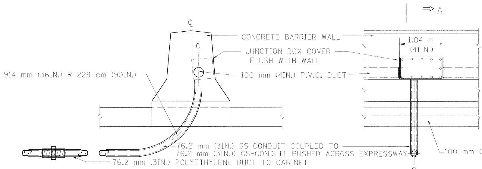
TYPE "J" JUNCTION BOX PLACEMENT WITH 76.2 mm (3IN.) GS-CONDUIT ACCESS
