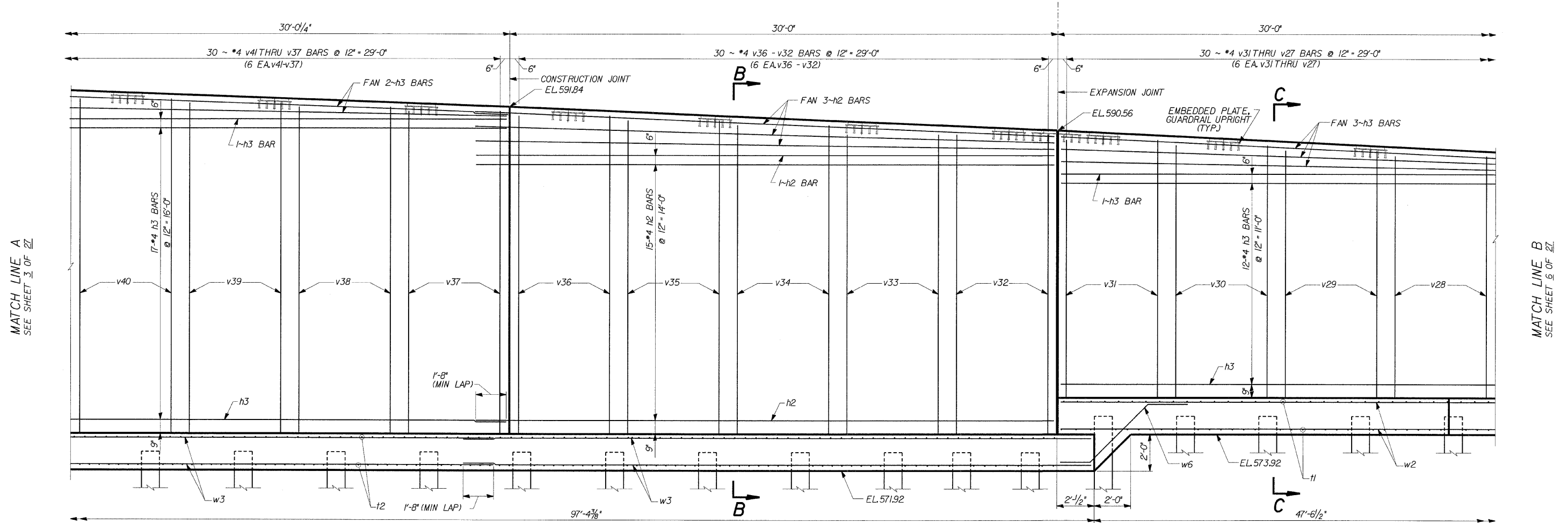
ELEVATION (SHOWING FRONT FACE REINFORCEMENT)
