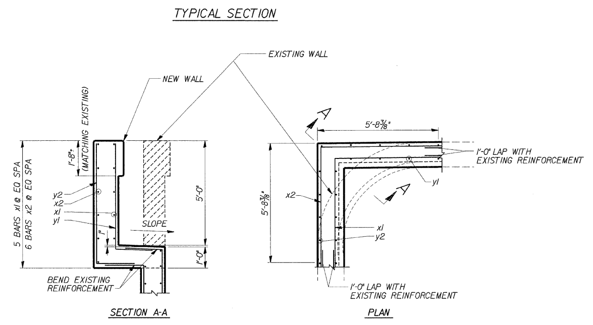
EXISTING RETAINING WALL SCALE: NOT TO SCALE AT RAMP F AND JACKSON BLVD.
