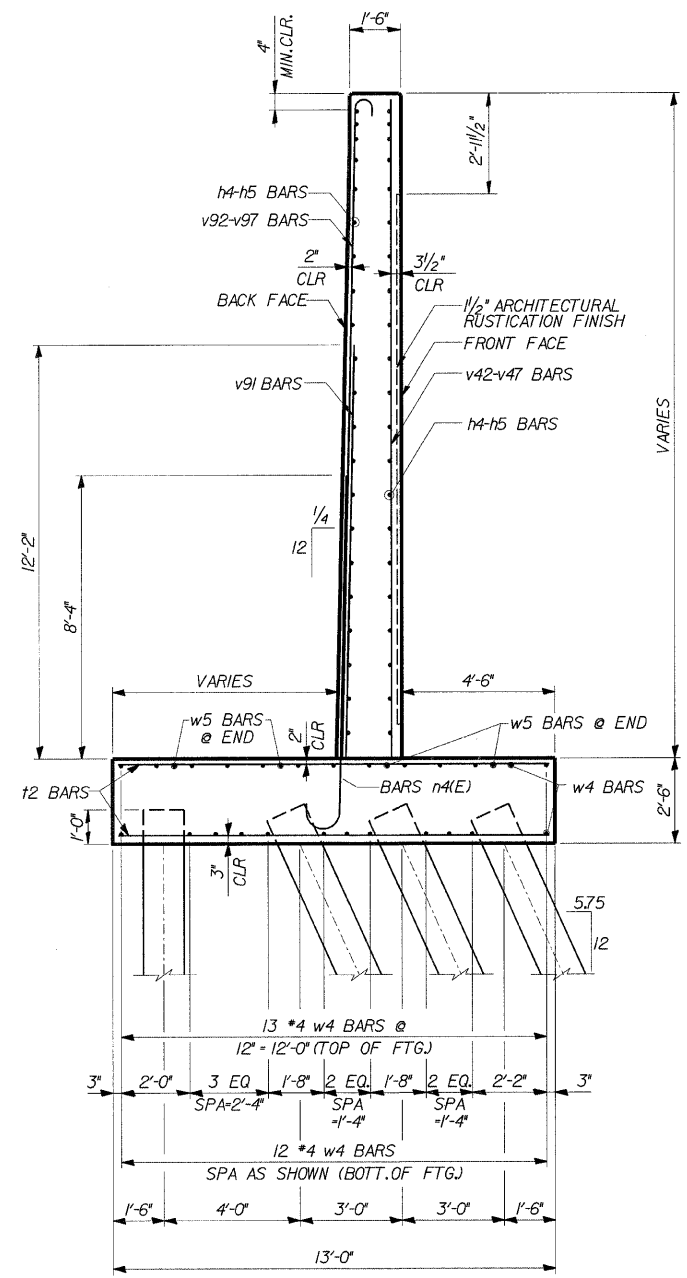
SECTION A-A STA. 13+09.42 THRU STA. 13+45.60 (FOR DETAILS NOT SHOWN SEE TYPICAL SECTION)
