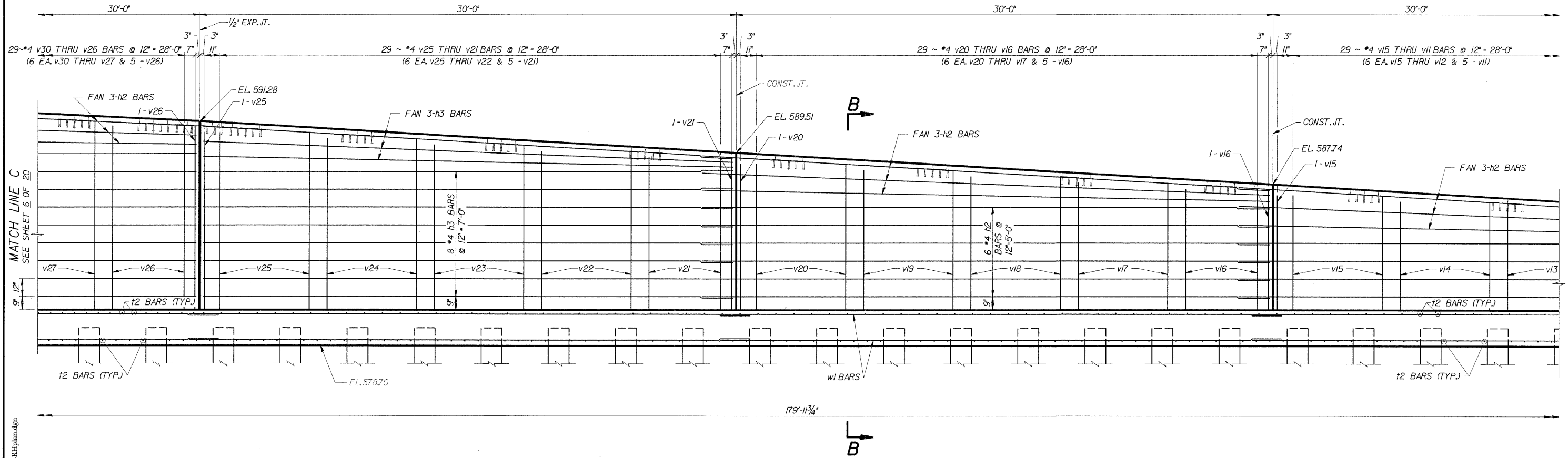
ELEVATION (SHOWING FRONT FACE REINFORCEMENT)
