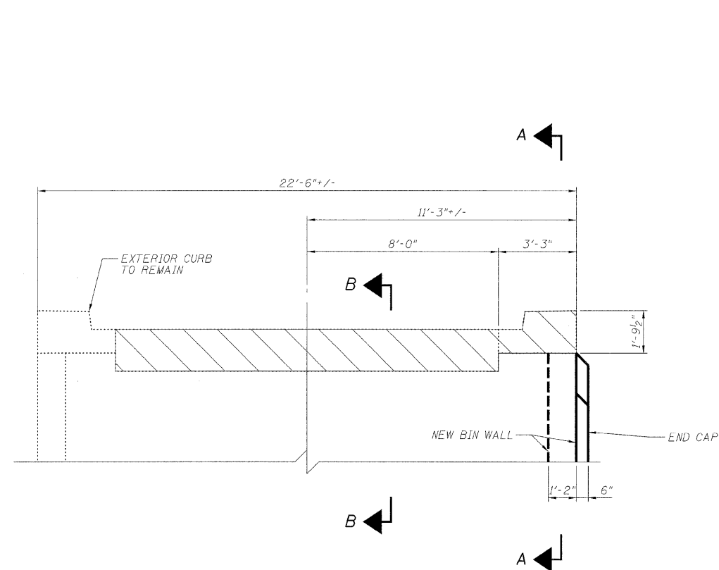
EXISTING ABUTMENT ELEVATION (LOOKING @ BACKFACE)
