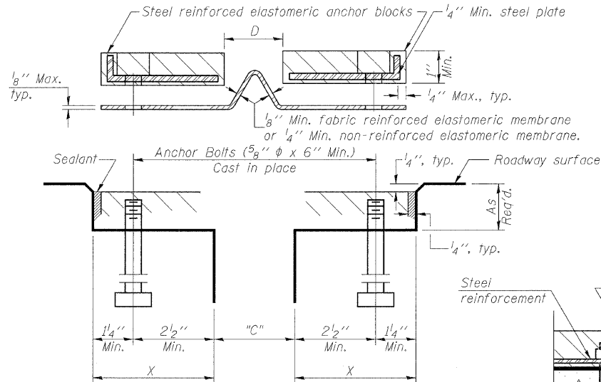
CROSS SECTION
