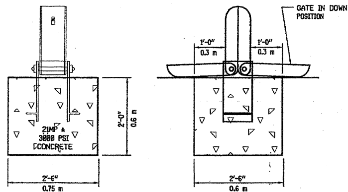
FRONT VIEW SIDE VIEW TIP DOWN GATE INSTALLATION DETAIL N.T.S.
