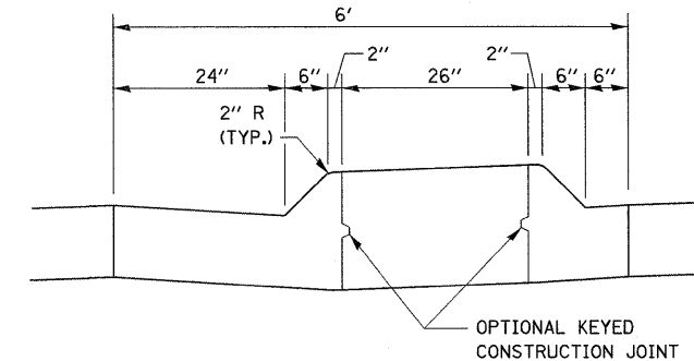
SOLID MEDIAN DETAIL SM-6.24 MEDIAN (SPECIAL) STA. 784+10.00 TO STA. 785+47.00
