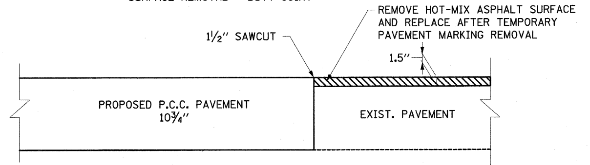
TRANSITION AT STA 507+90
