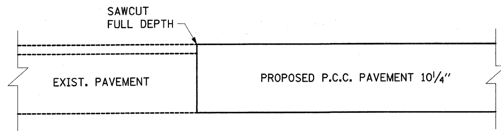
TRANSITION AT STA 1325+65
