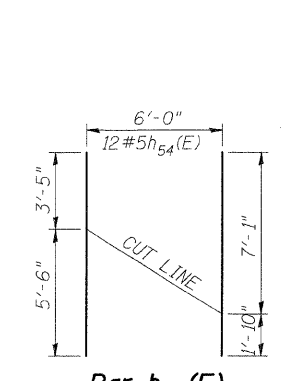
Bar h 54 (E) CUTTING DIAGRAM
