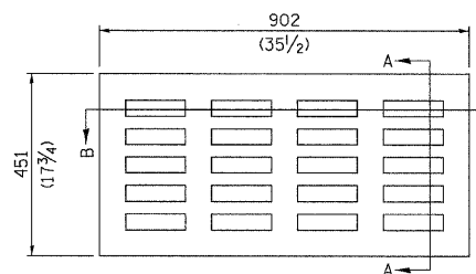
PLAN OF GRATE
