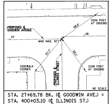
STA. 27+69.78 BK. (CL GOODWIN AVE.) = STA. 400+03.10 (CL ILLINOIS ST.)
