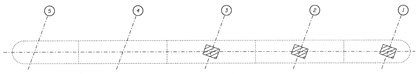
PLAN - PIER NO. 5 (0.45 cu ft of non-shrink grout)
