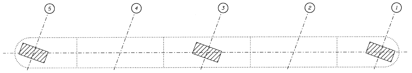
PLAN - PIER NO. 3 (0.65 cu ft of non-shrink grout)
