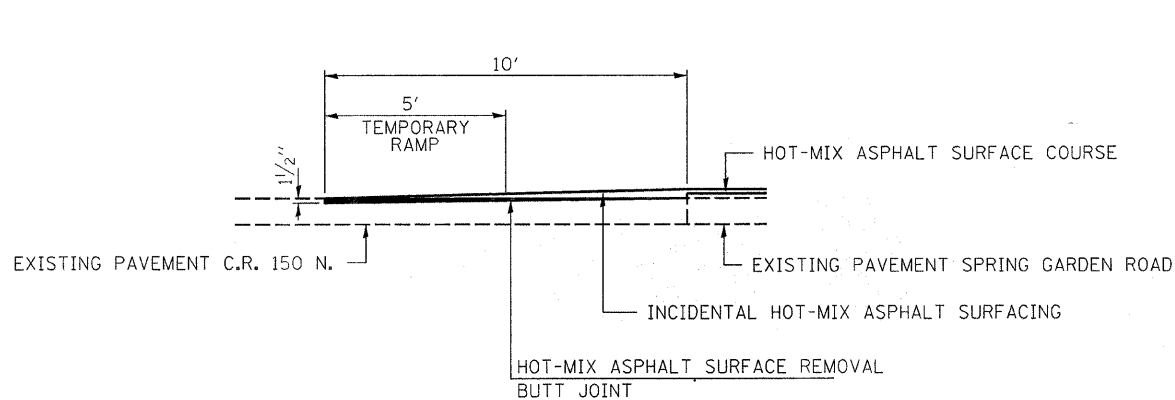
C.R. 150 N. / SPRNG GARDEN ROAD TIE-IN
