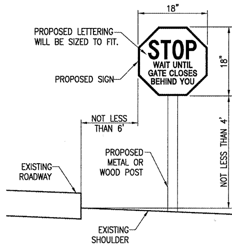
TYPICAL SLIDE GATE STOP SIGN
