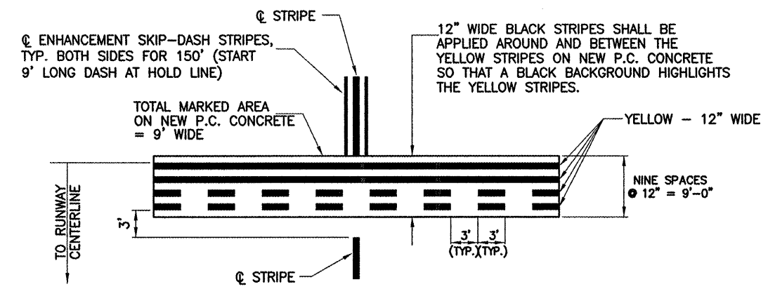
DETAIL B HOLDING LINE MARKINGS
