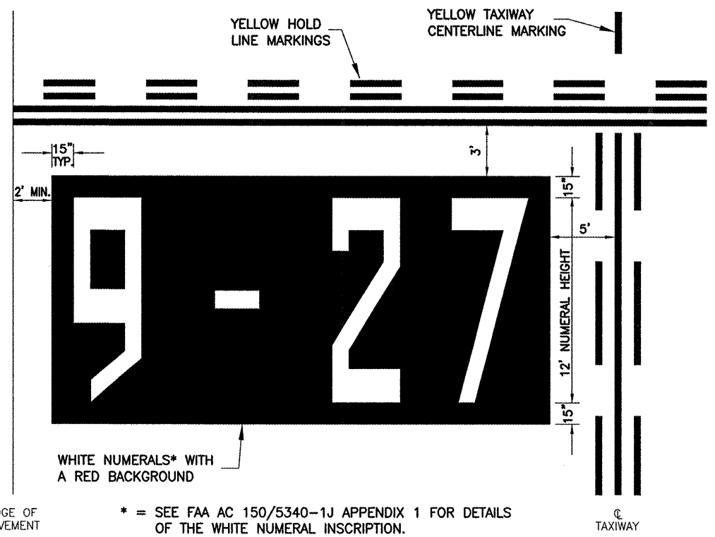
DETAIL D PAINTED SURFACE HOLDING POSITION SIGN
