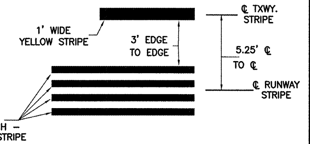
DETAIL C RUNWAY CL / TAXIWAY CL STRIPES
