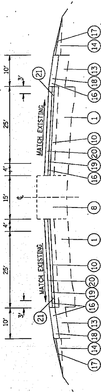
TYPICAL SECTION MILE 0.00 TO MILE 0.55
