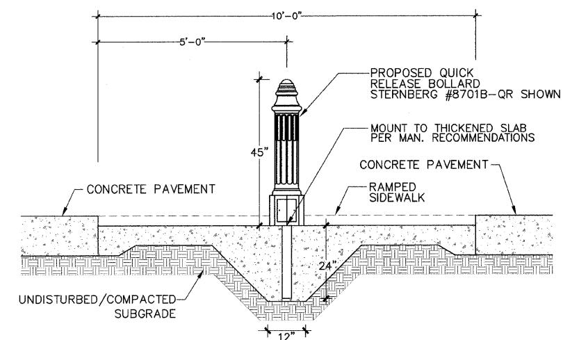
E - TYPICAL QUICK RELEASE BOLLARD CROSS SECTION
