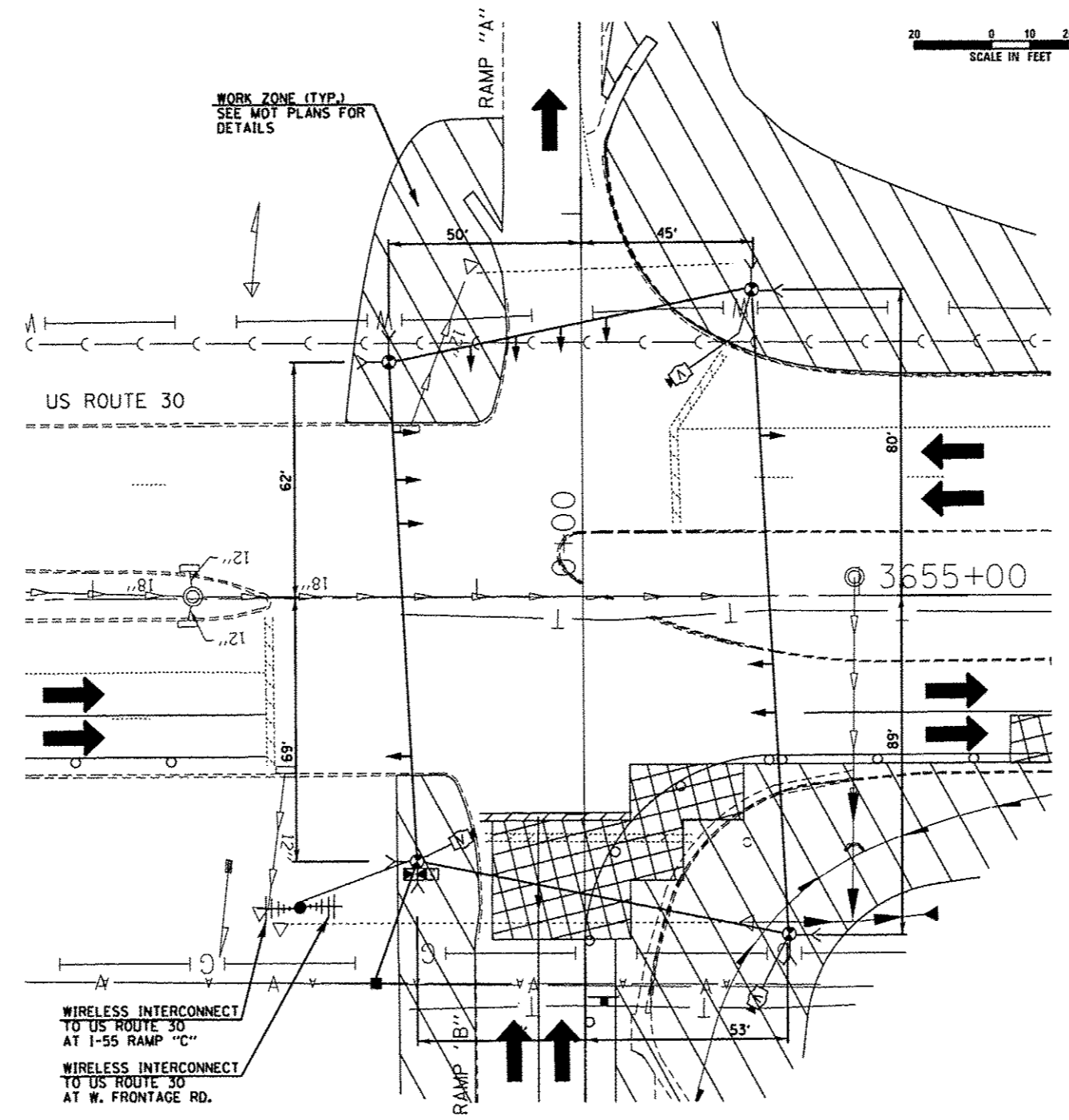
SIGNAL HEAD PLACEMENT FOR STAGE I
