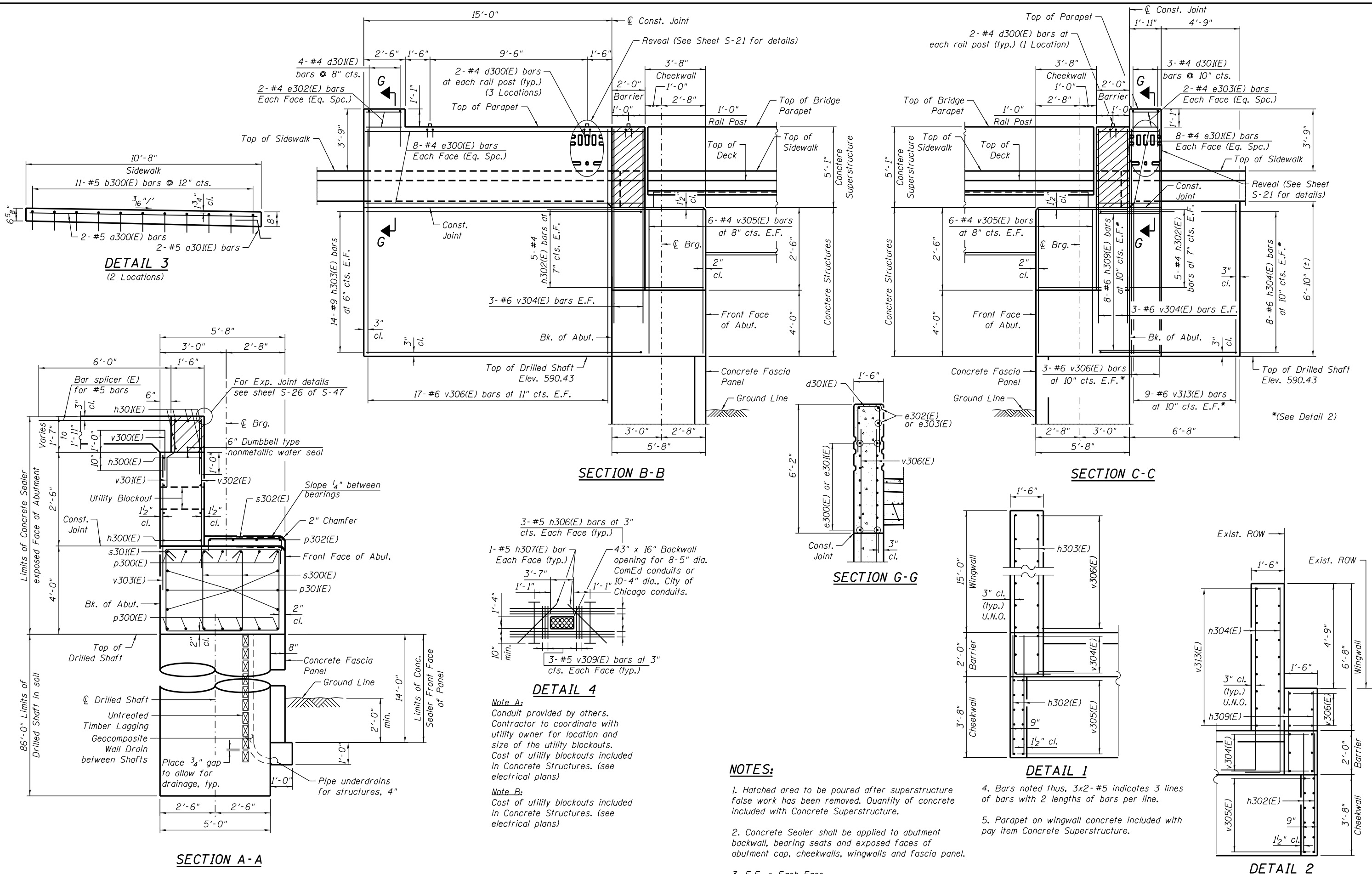
DETAIL 2
