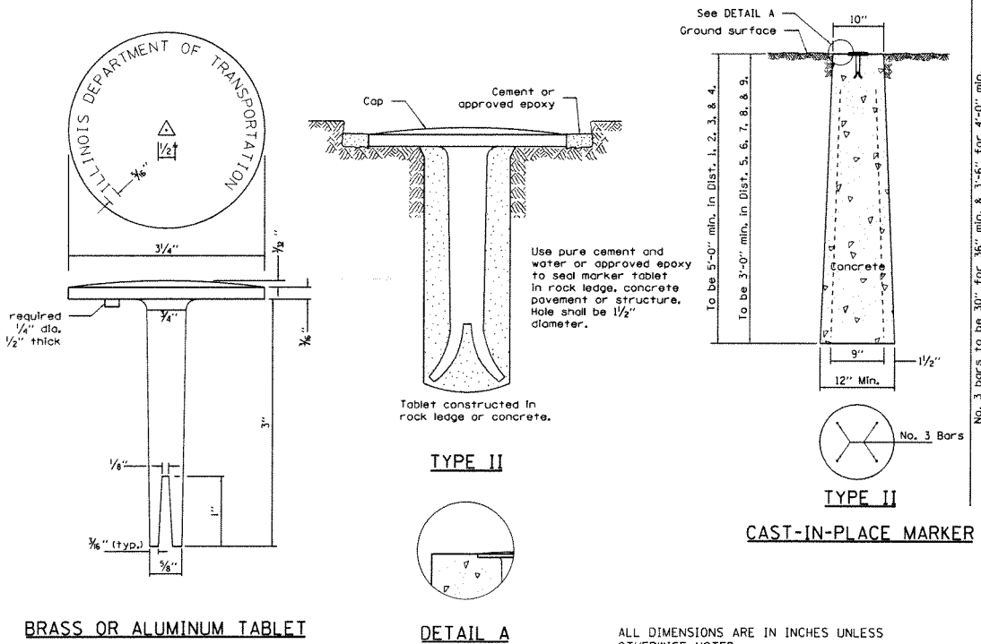
DETAIL A
