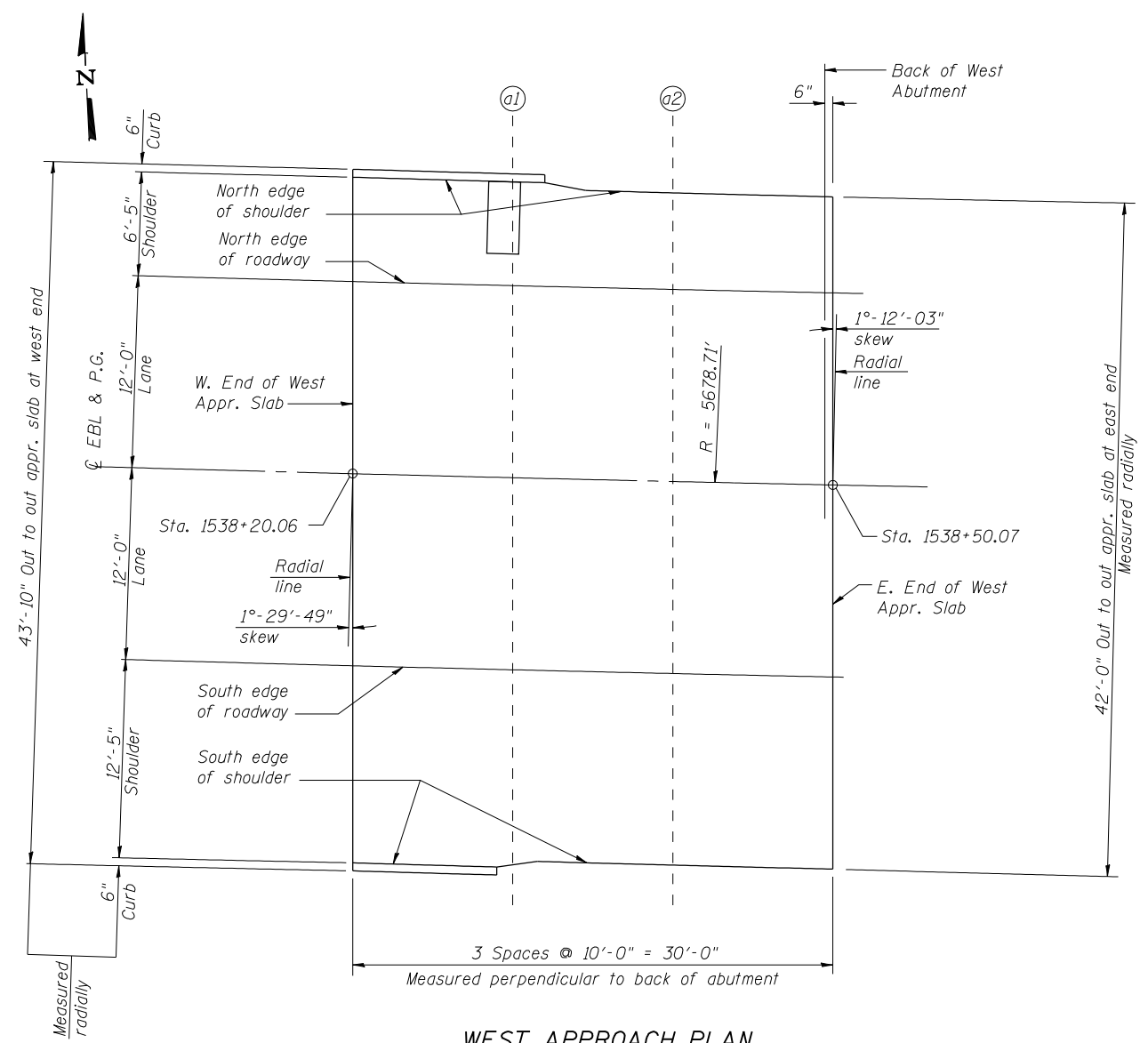
WEST APPROACH PLAN
