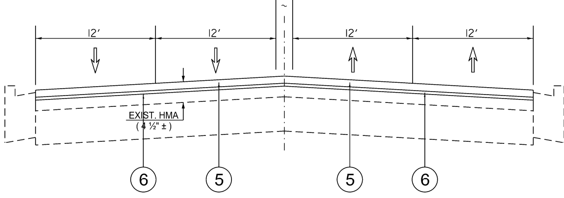
PROP. TYPICAL SECTION
