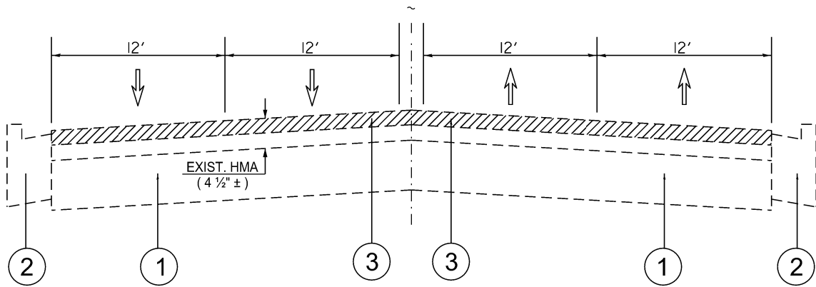
EXIST. TYPICAL SECTION
