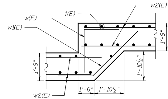
STEP DETAIL
