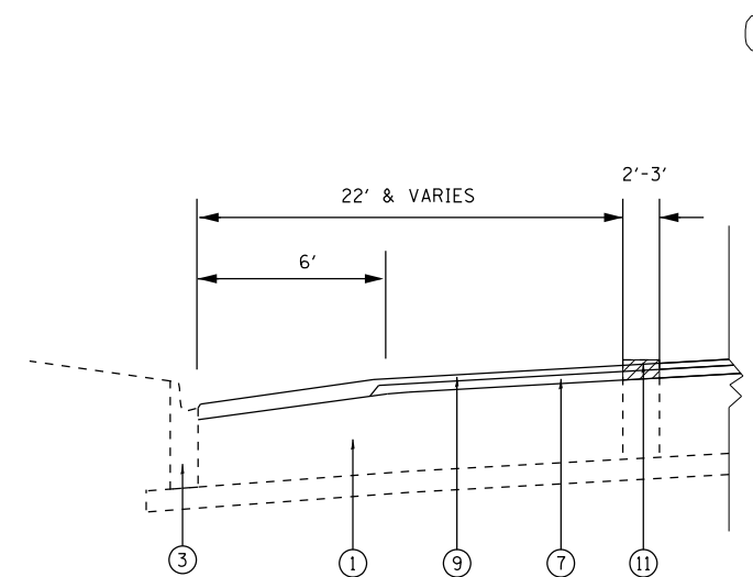
PROPOSED MEDIAN REMOVAL, PARTIAL DEPTH (TO BE OVERLAID AND REPLACED WITH THERMOPLASTIC PAVEMENT MARKING - LINE 6" (TYP))
