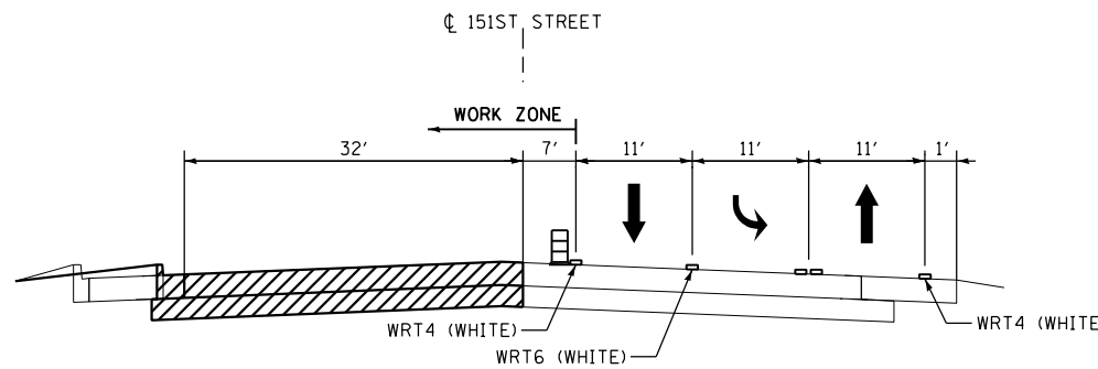
151ST STREET TYPICAL SECTION - STAGE B (EAST OF LAGRANGE)
