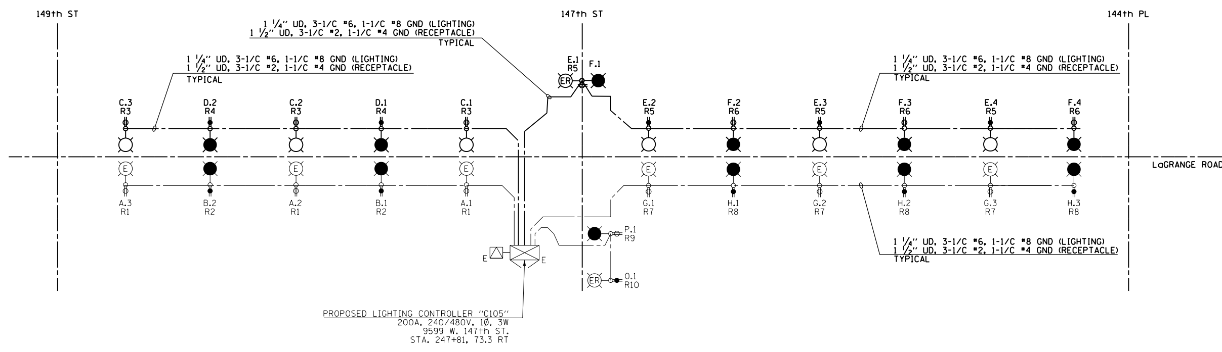
LIGHTING CONTROLLER "C105" STAGE 3 WIRING DIAGRAM N.T.S.
