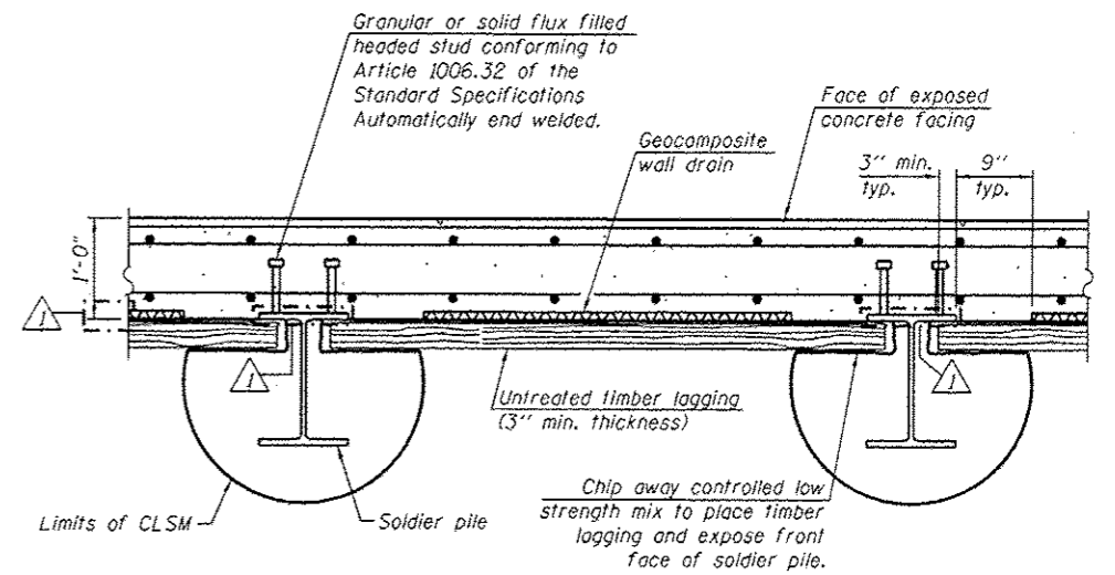
DETAIL PLAN
