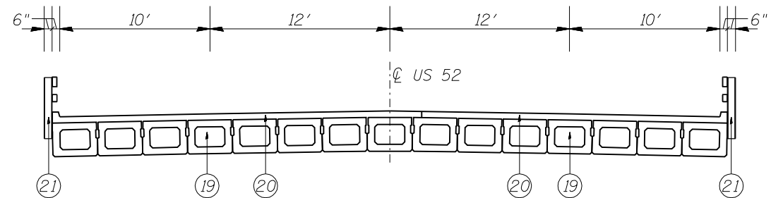
PROPOSED TYPICAL SECTION STA. 452+26.87 TO STA. 452+89.22
