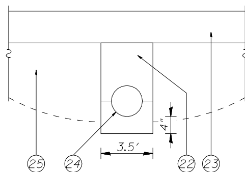
PROPOSED DRIVEWAY SECTION STA. 448+82 TO STA. 449+18
