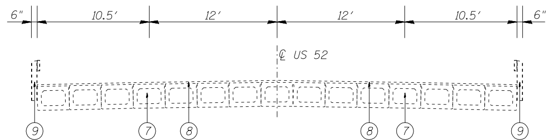
EXISTING TYPICAL SECTION STA. 452+26.87 TO STA. 452+89.22
