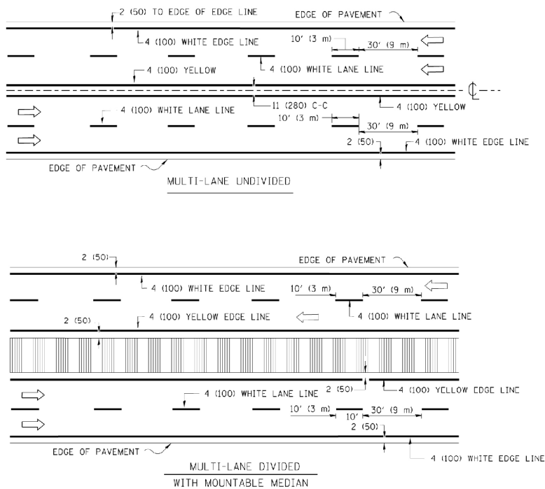
TYPICAL LANE AND EDGE LINE MARKING
