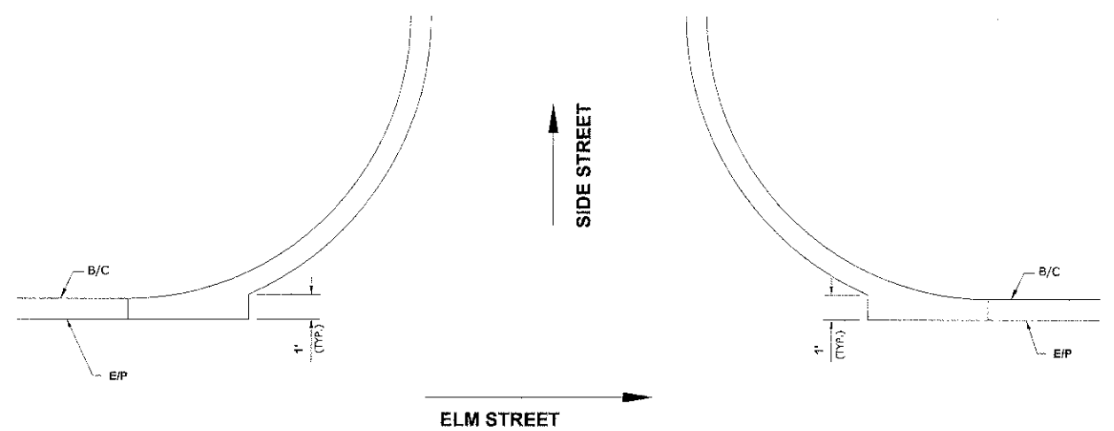
TYPICAL 1' STRAIGHT EXTENSION AT INTERSECTIONS
