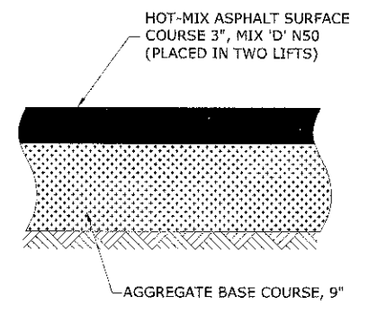
INCIDENTAL HOT-MIX ASPHALT SURFACING (TYPICAL ASPHALT PARKING)
