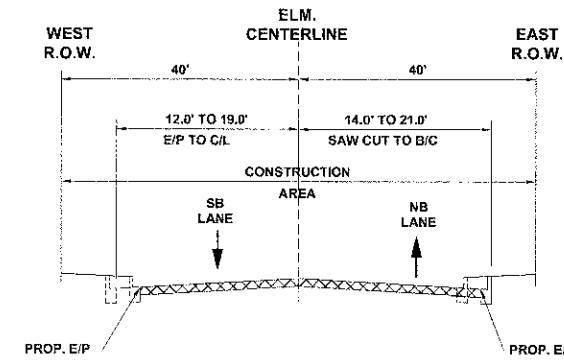
STAGE 1 CONSTRUCTION TYPICAL SECTION
