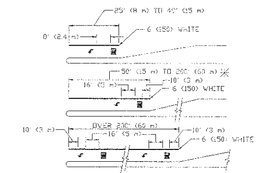
TYPICAL TURN LANE MARKING
