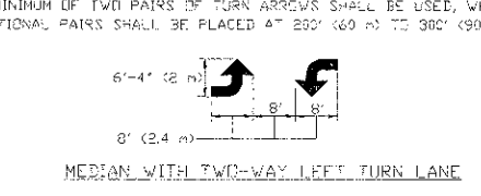
TYPICAL TURN LANE MARKING
