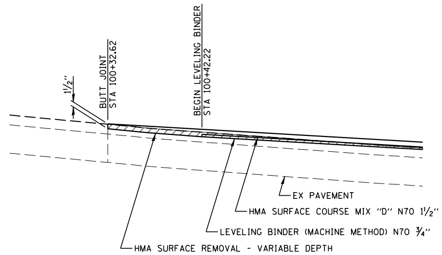
BUTT JOINT DETAIL 6TH ST RD
