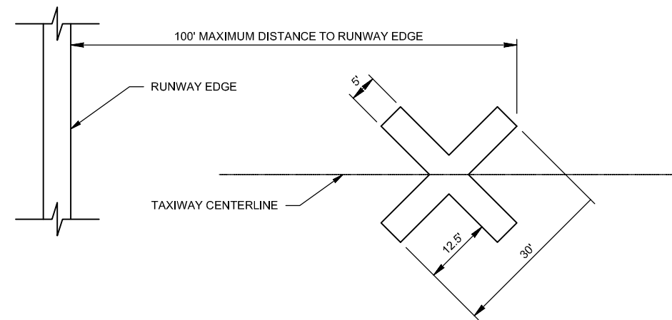
TYPICAL TAXIWAY CLOSURE MARKER DETAIL N.T.S.
