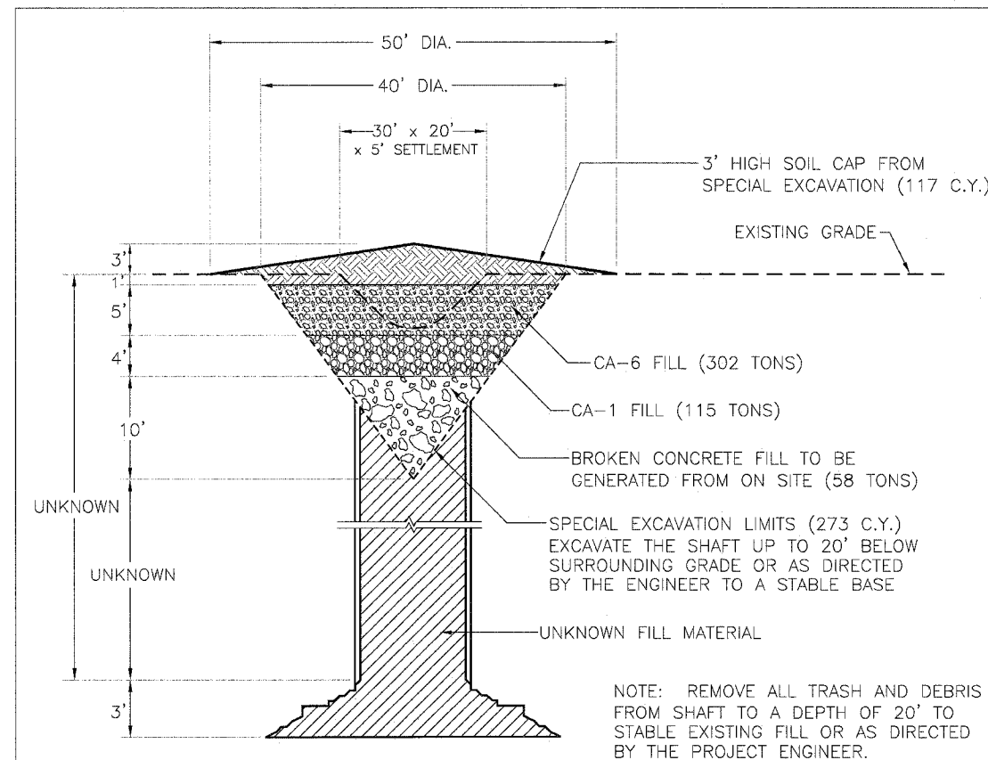
D GARY COAL COMPANY SHAFT 12 NOT TO SCALE
