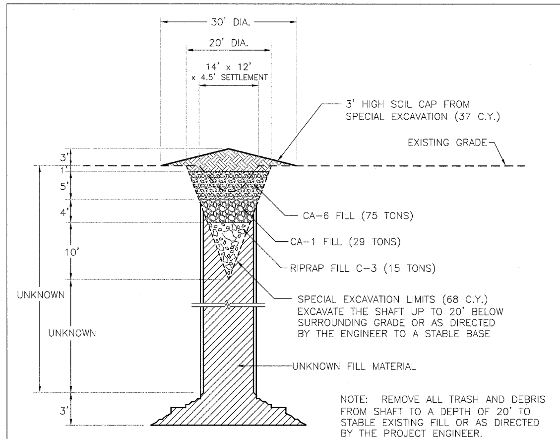
A MAPLETON MINE SHAFT 12 NOT TO SCALE
