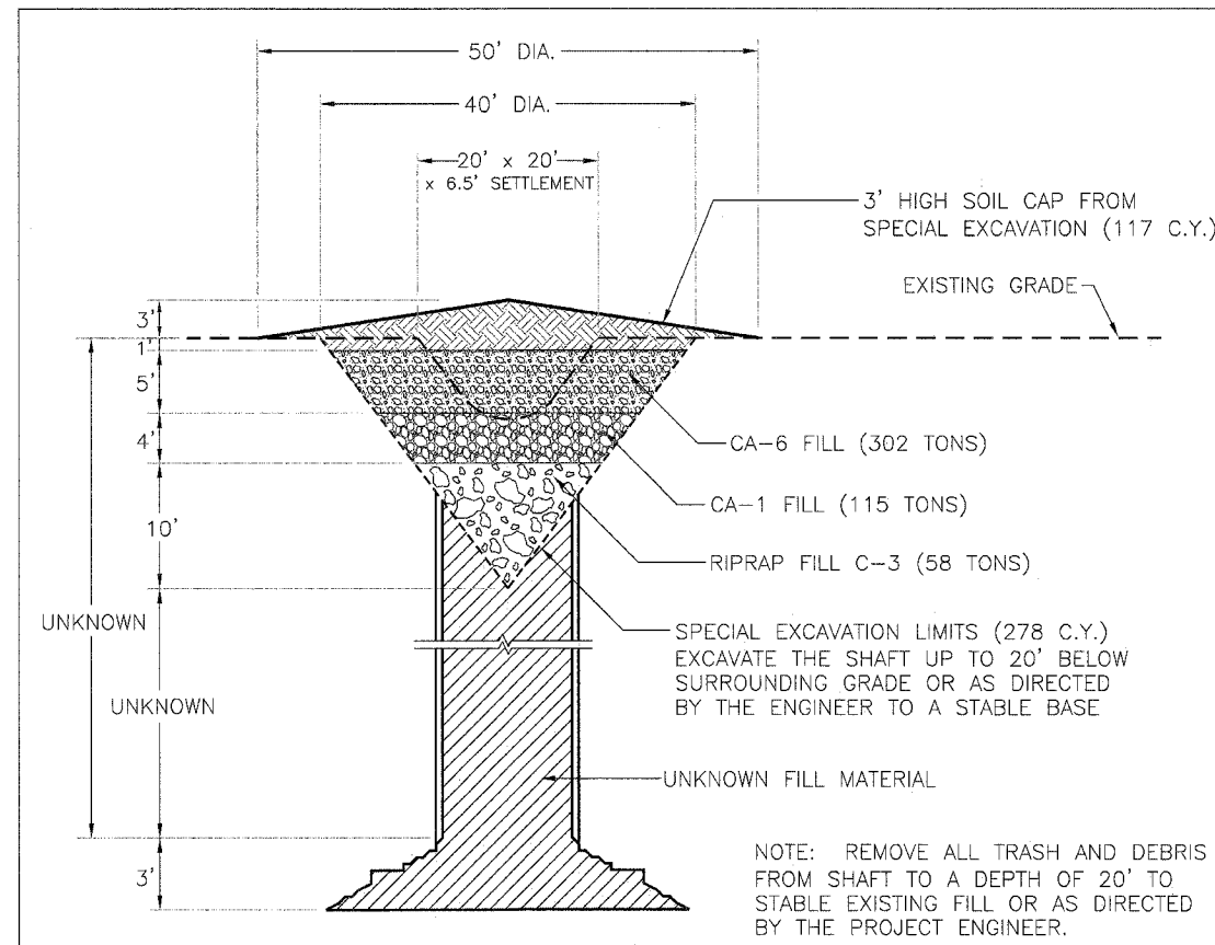
B MAPLETON MINE SHAFT 12 NOT TO SCALE
