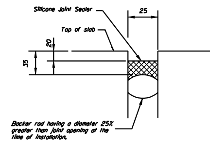
LONGITUDINAL OPEN JOINT (SB ROADWAY ONLY)
