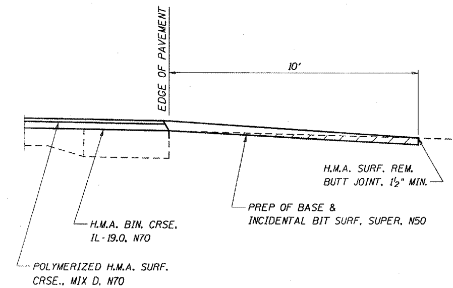
SECTION C-C FOR BITUMINOUS SIDEROAD
