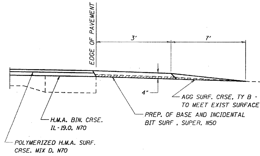
SECTION A-A FOR AGG P.E.
