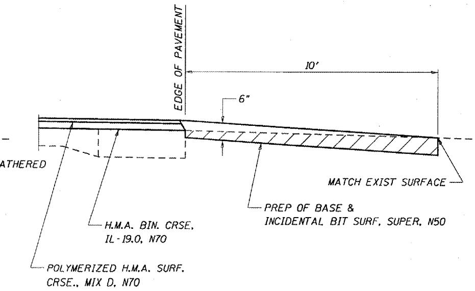
SECTION B-B FOR OIL & CHIP SIDEROAD
