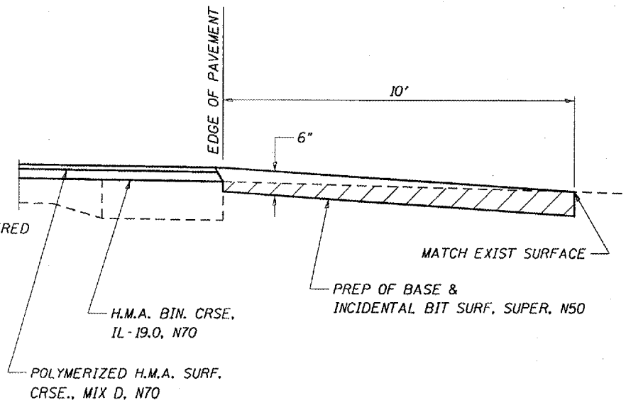
SECTION B-B FOR OIL & CHIP SIDEROAD
