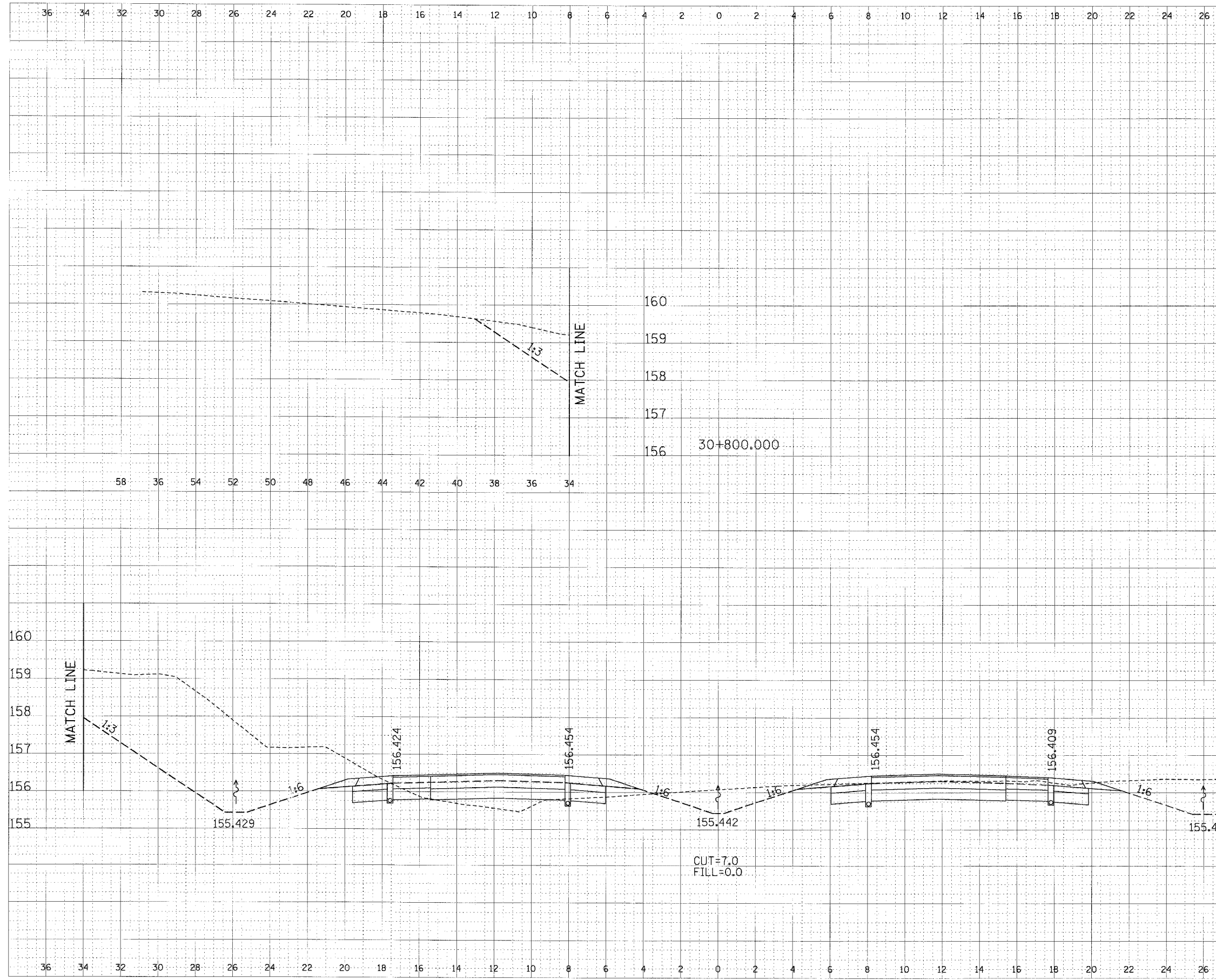
CROSS SECTION, FAP ROUTE 310, STA 30+800.000
