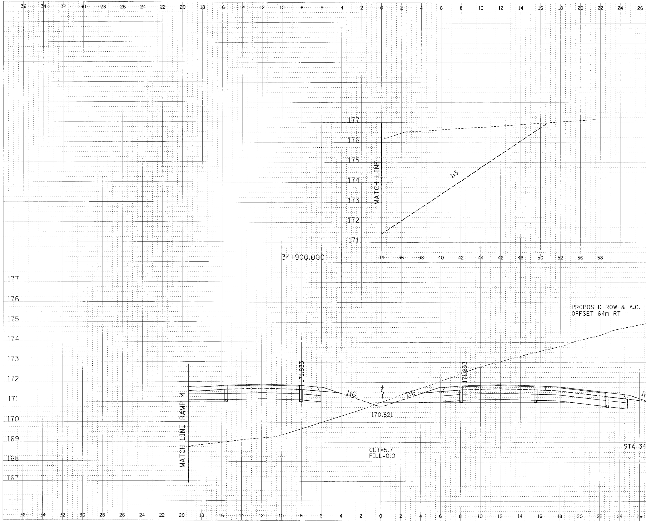
CROSS SECTION, FAP ROUTE 310, STA 34+900.000
