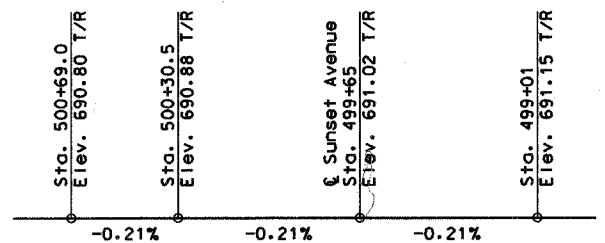
RAILWAY PROFILE T/R
