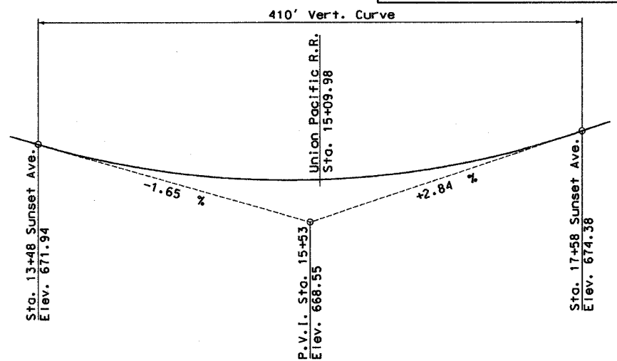
SUNSET AVE. PROFILE
