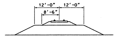
EXISTING EMBANKMENT
